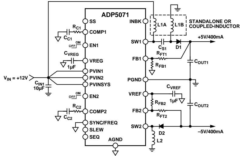
Figure 48. SEPIC Application for +12 V in to ±5 V Output Generation
