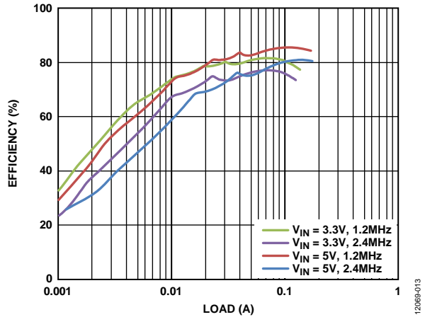
Figure 13. Inverting Regulator Efficiency vs. Current Load, V_{NEG} = -15V , T_A = 25^\circ C
