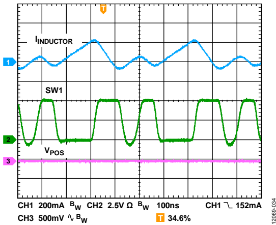
Figure 34. Boost Regulator Discontinuous Conduction Mode Operation Showing Inductor Current ( I_{INDUCTOR} ), Switch Node Voltage, and Output Ripple, V_{IN} = 5V , V_{POS} = 15V , I_{LOAD1} = 35mA , f_{SW} = 2.4MHz , T_A = 25^\circ C
