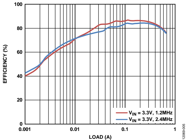
Figure 5. Boost Regulator Efficiency vs. Current Load, V_{IN} = 3.3 V, V_{POS} = 5 V, T_A = 25^\circ\text{C}
