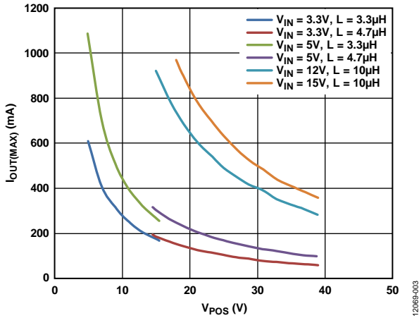
Figure 3. Boost Regulator Maximum Output Current, f_{SW} = 1.2 MHz, T_A = 25^\circ\text{C} , Based on Target of 70% I_{LIM(BOOST)}
