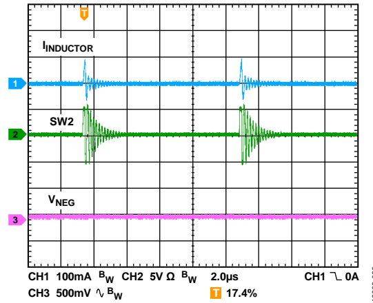
Figure 36. Inverting Regulator Skip Mode Operation Showing Inductor Current ( I_{INDUCTOR} ), Switch Node Voltage, and Output Ripple, V_{IN} = 5V , V_{NEG} = -15V , I_{LOAD2} = 1mA , f_{SW} = 2.4MHz , T_A = 25^\circ C
