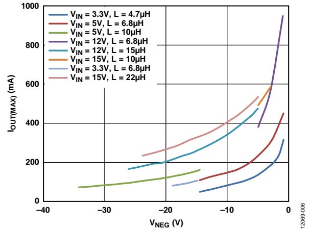
Figure 6. Inverting Regulator Maximum Output Current, f_{SW} = 1.2 MHz, T_A = 25^\circ\text{C} , Based on Target of 70% I_{LIM(INVERTER)}
