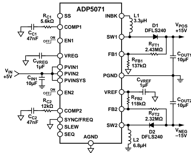
Figure 46. Typical +5 V to \pm 15 V Application
