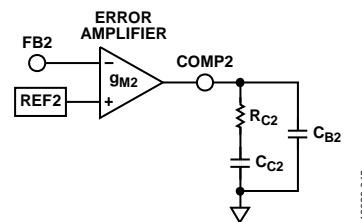
Figure 45. Compensation Component
