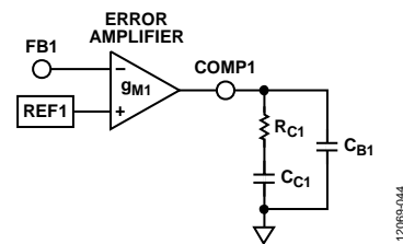
Figure 44. Compensation Components
