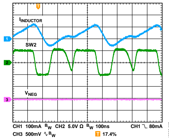
Figure 37. Inverting Regulator Discontinuous Conduction Mode Operation Showing Inductor Current ( I_{INDUCTOR} ), Switch Node Voltage, and Output Ripple, V_{IN} = 5V , V_{NEG} = -15V , I_{LOAD2} = 6mA , f_{SW} = 2.4MHz , T_A = 25^\circ C
