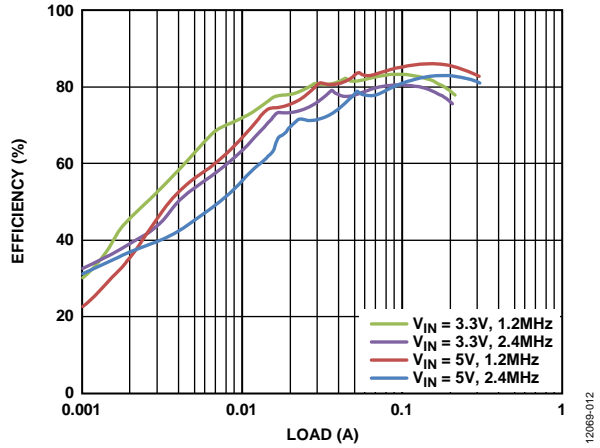
Figure 12. Inverting Regulator Efficiency vs. Current Load, V_{NEG} = -9V , T_A = 25^\circ C
