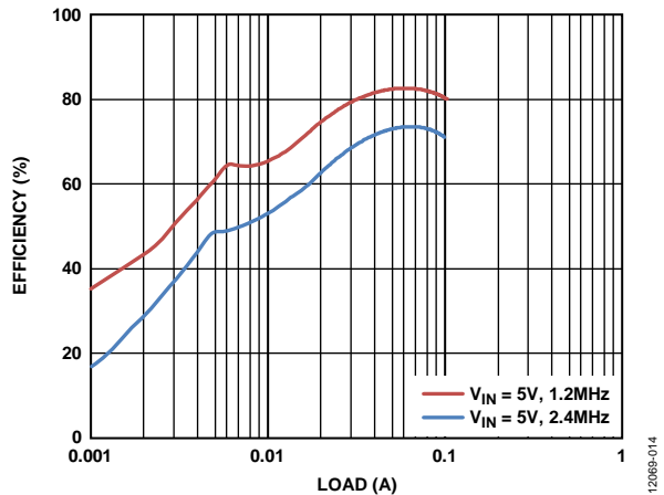
Figure 14. Inverting Regulator Efficiency vs. Current Load, V_{NEG} = -34V , T_A = 25^\circ C
