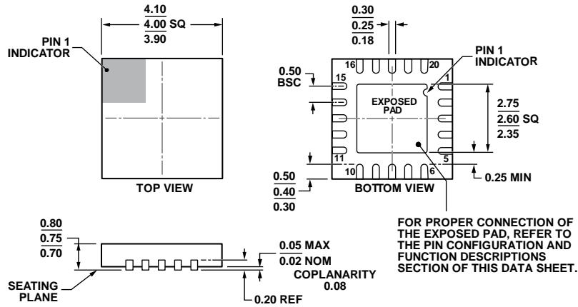
Figure 50. 20-Lead Lead Frame Chip Scale Package [LFCSP_WQ] 4 mm × 4 mm Body, Very Very Thin Quad (CP-20-8) Dimensions shown in millimeters
