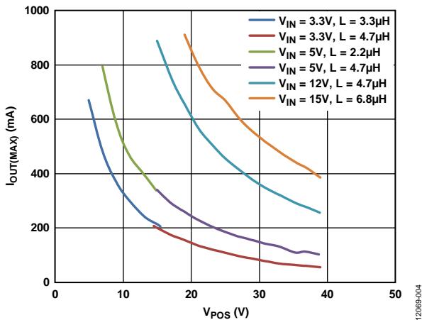
Figure 4. Boost Regulator Maximum Output Current, f_{SW} = 2.4 MHz, T_A = 25^\circ\text{C} , Based on Target of 70% I_{LIM(BOOST)}
