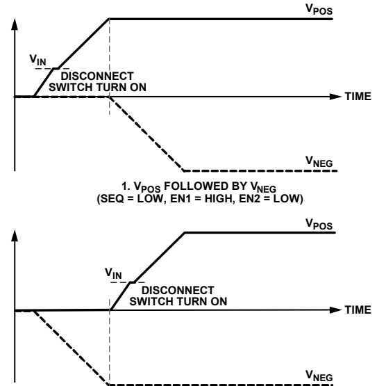
Figure 42. Sequential Enable Mode
