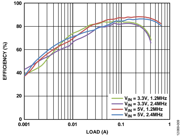
Figure 9. Boost Regulator Efficiency vs. Current Load, V_{POS} = 9V , T_A = 25^\circ C
