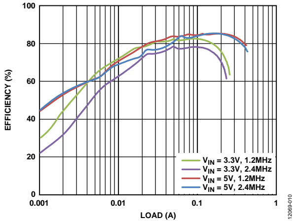
Figure 10. Boost Regulator Efficiency vs. Current Load, V_{POS} = 15V , T_A = 25^\circ C
