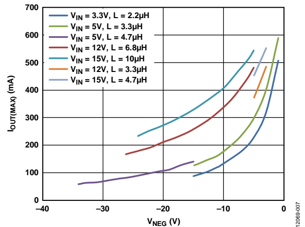
Figure 7. Inverting Regulator Maximum Output Current, f_{SW} = 2.4 MHz, T_A = 25^\circ\text{C} , Based on Target of 70% I_{LIM(INVERTER)}
