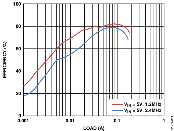
Figure 11. Boost Regulator Efficiency vs. Current Load, V_{POS} = 34V , T_A = 25^\circ C
