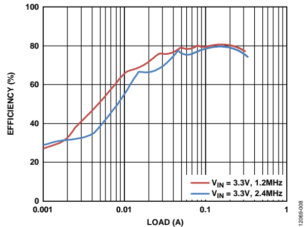
Figure 8. Inverting Regulator Efficiency vs. Current Load, V_{IN} = 3.3 V, V_{NEG} = -5 V, T_A = 25^\circ\text{C}
