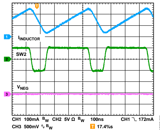
Figure 38. Inverting Regulator Continuous Conduction Mode Operation Showing Inductor Current ( I_{INDUCTOR} ), Switch Node Voltage, and Output Ripple, V_{IN} = 5V , V_{NEG} = -15V , I_{LOAD2} = 35mA , f_{SW} = 2.4MHz , T_A = 25^\circ C
