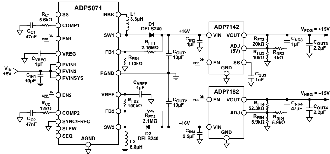
Figure 47. Super Low Noise \pm 15\text{ V} Generation with Post Regulation by the ADP7142 ( +40\text{ V} , +200\text{ mA} , Low Noise LDO) and ADP7182 ( -28\text{ V} , -200\text{ mA} , Low Noise LDO)
